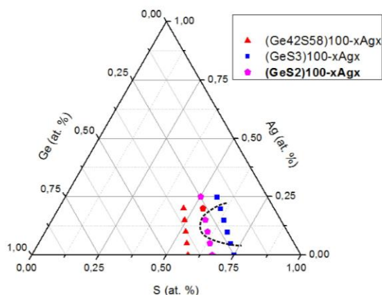
Fig. 5. Area of phase separation of Ge-S-Ag glasses
