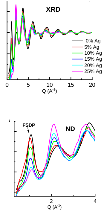
Fig. 2. XRD and ND structure factors (\text{GeS}_3)_{100-x}\text{Ag}_x glasses
